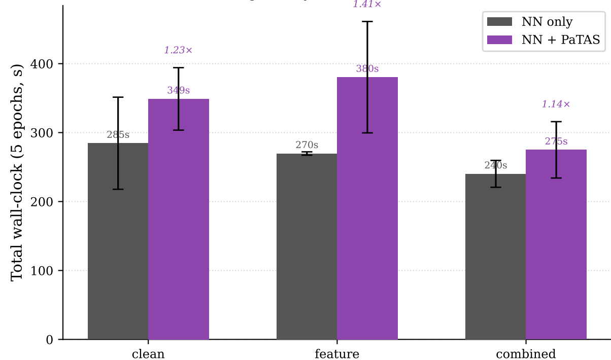
Training latency across noise conditions
